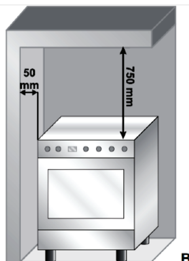
Free-standing installation
